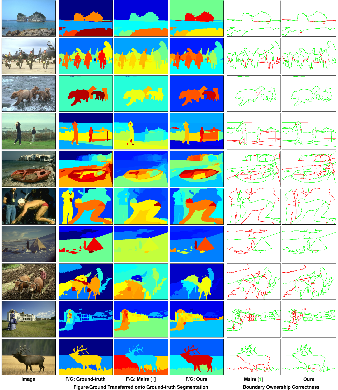
Figure 1. Figure/ground predictions measured on ground-truth segmentation. We transfer per-pixel figure/ground predictions (columns 2 through 4 of Figure 7 in the paper) onto the ground-truth segmentation by taking the median value over each region. For boundaries separating regions with different ground-truth figure/ground layer assignments, we check whether the predicted owner (more figural region) matches the owner according to the ground-truth. The rightmost two columns mark correct boundary ownership predictions in green and errors in red for both the results of Maire’s system [1] and our system. Note how we correctly predict ownership of object lower boundaries (rows 6, 8, 10) and improve on small objects (row 7). Table 1 gives quantitative benchmarks.
