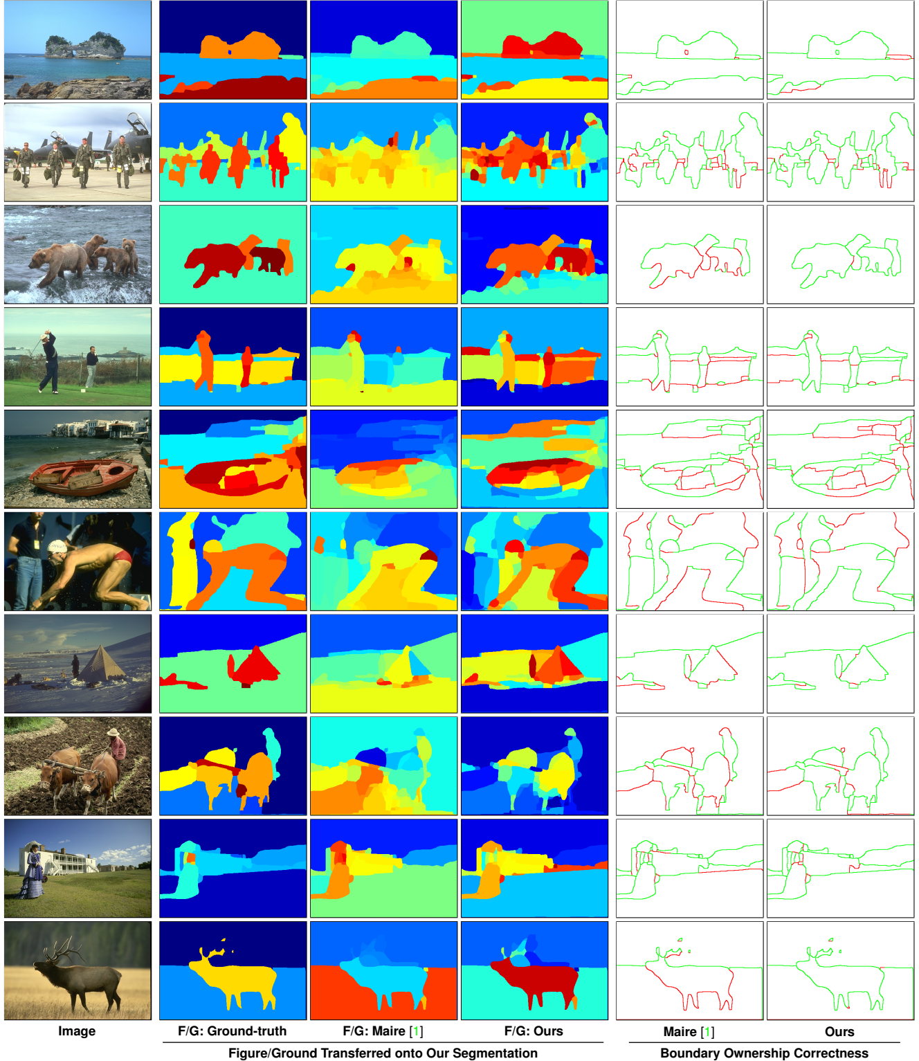
Figure 2. Figure/ground predictions measured on our segmentation. As in Figure 1, we transfer ground-truth figure/ground, Maire’s figure/ground predictions [1], and our predictions onto a common segmentation. However, instead of using the ground-truth segmentation, we transfer onto the segmentation generated by our system. The ground-truth figure/ground transferred onto our regions defines the boundary ownership signal against which we judge predictions. Comparing with Figure 1, our boundary ownership predictions are mostly consistent regardless of the segmentation (ground-truth or ours) to which they are applied. However, row 3 shows this is not the case for [1]; here, its predicted correct ownership for the lower boundary relies on averaging out over a large ground-truth background region.
