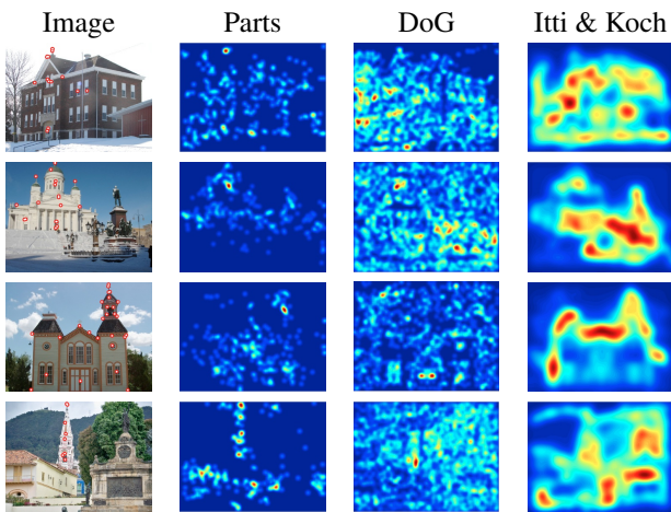
Figure 9. From left to right – images shown with the landmarks; saliency maps from our parts, Difference of Gaussian (DoG) inter-point operator, and the Itti and Koch model.
