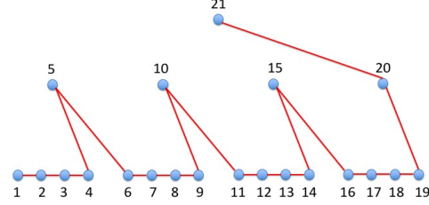
Figure 3: The edge set E_2 in G_{4,2} (only a single copy of each edge is shown).
