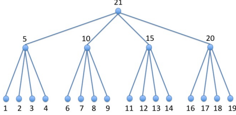
Figure 2: Tree T_{4,2} with vertices indexed according to post-order traversal.
