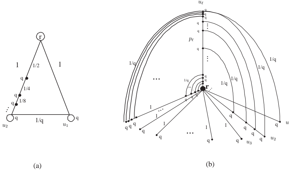
Fig. 2. (a) Price of anarchy of 2 - \epsilon . (b) Price of anarchy of \Omega(\frac{\log n}{\log \log n}) .
