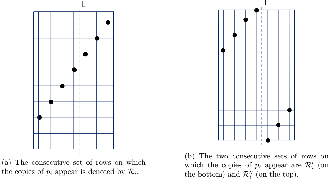
Figure 6: Two patterns in which copies of p_i may appear on strip S .
