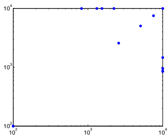
Figure 2. Learned [\sigma_1, \sigma_2] parameters of the kernels in the optimal convex combination, for the odd vs. even task. The parameter range was [100, 10000] .
