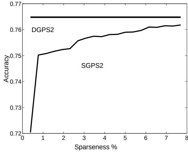
Figure 5.2: Test accuracy of Pitch Accent Prediction w.r.t. the sparseness of GPS solution.
