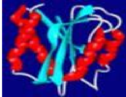
Figure 1.1: Three-dimensional structure of a protein
