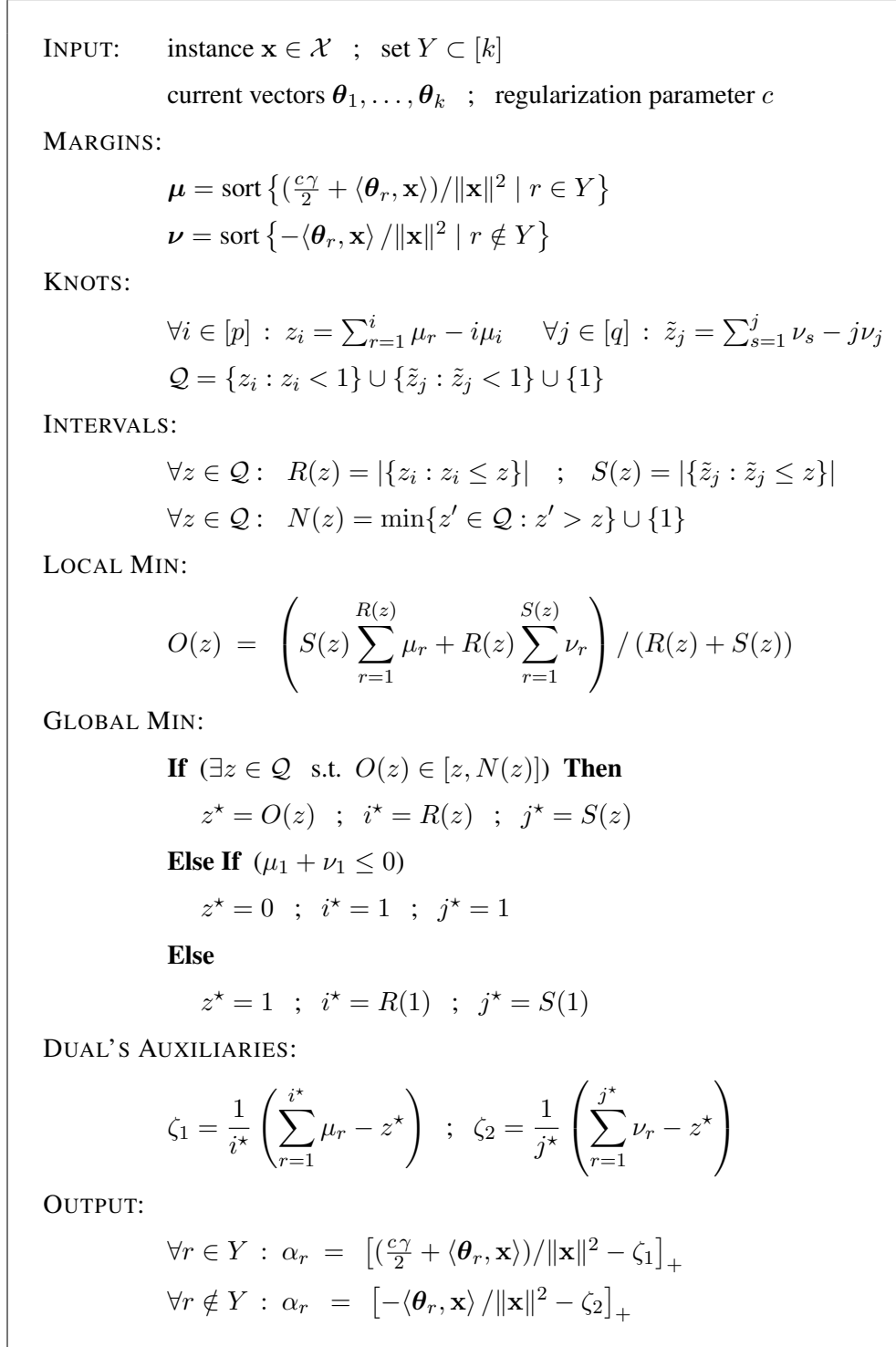
Figure 7.4: Pseudo-code for solving Eq. (7.18) when f(\mathbf{w}) = \frac{1}{2} \|\mathbf{w}\|^2 .
